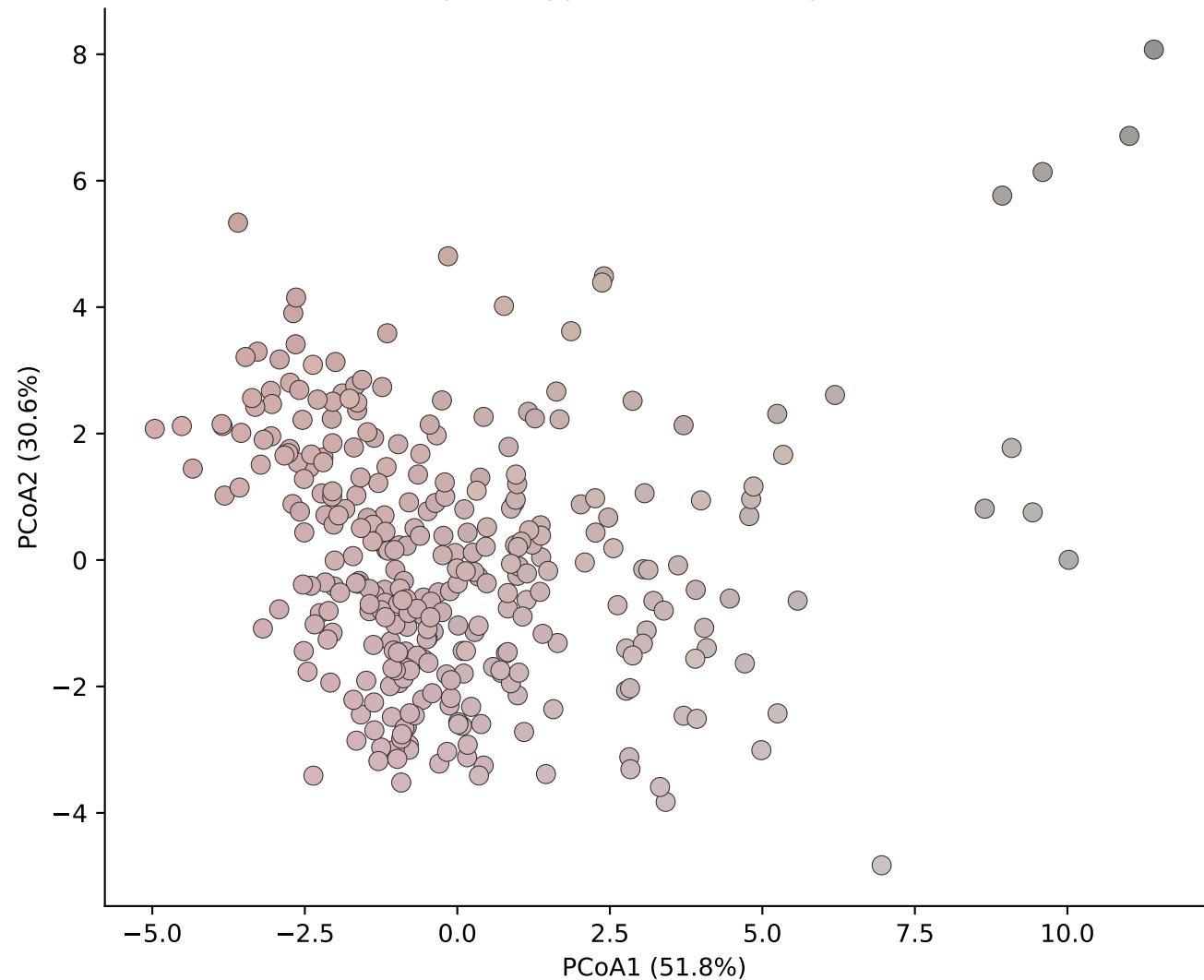
PCoA of CIELAB color phenotype ( L^* , a^* , b^* ) -- point = strain's own color
