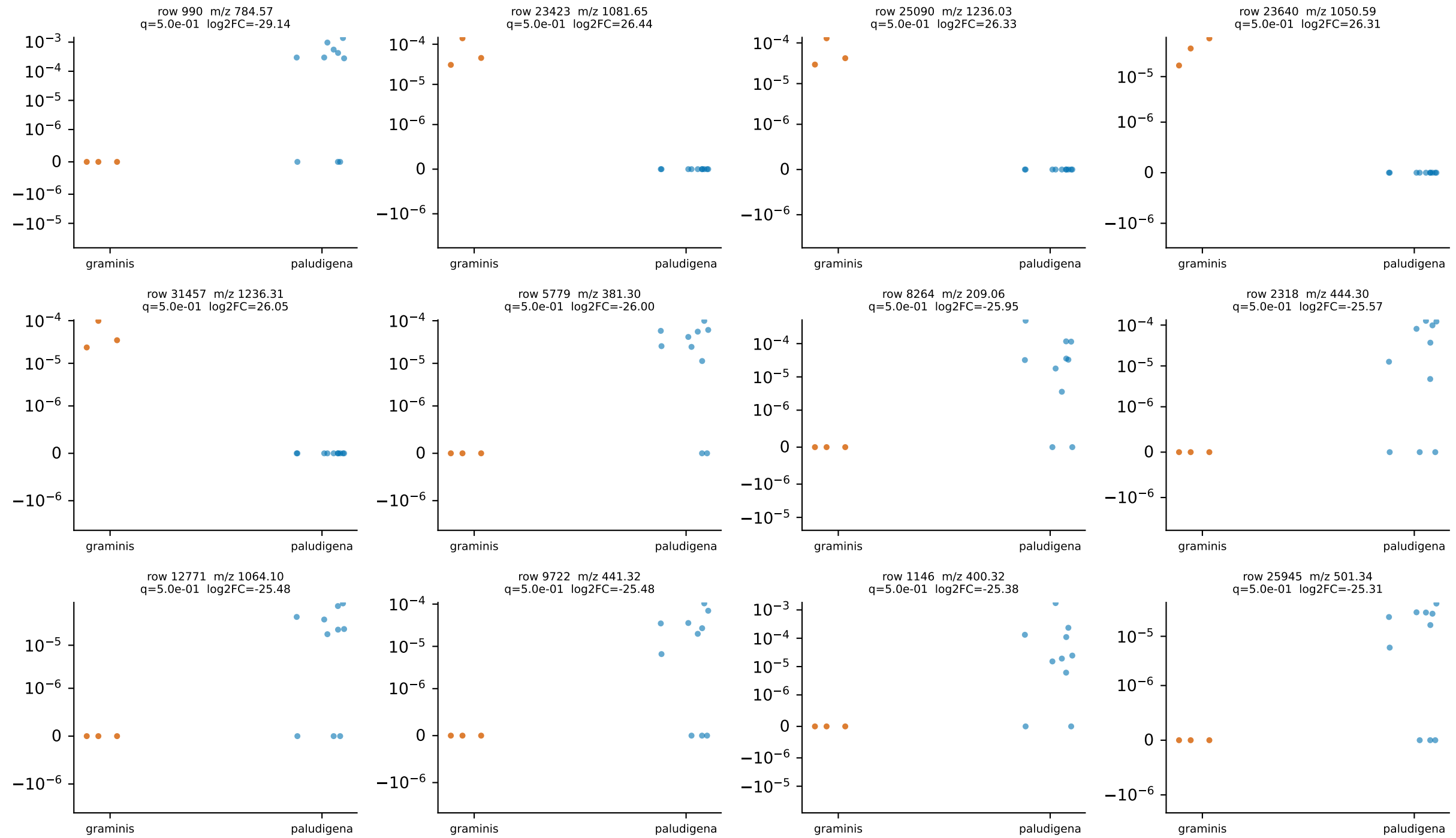
Top 12 differential features: Rhodotorula graminis vs Rhodotorula paludigena (TSS proportion, symlog y)
