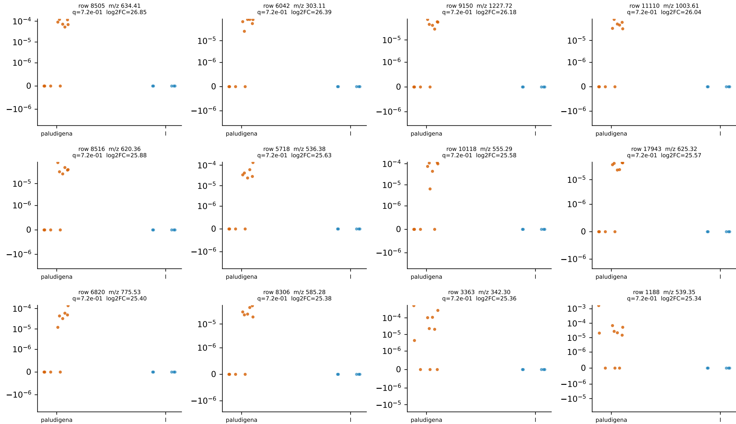
Top 12 differential features: Rhodotorula paludigena vs Rhodotorula sp. clade I (TSS proportion, symlog y)
