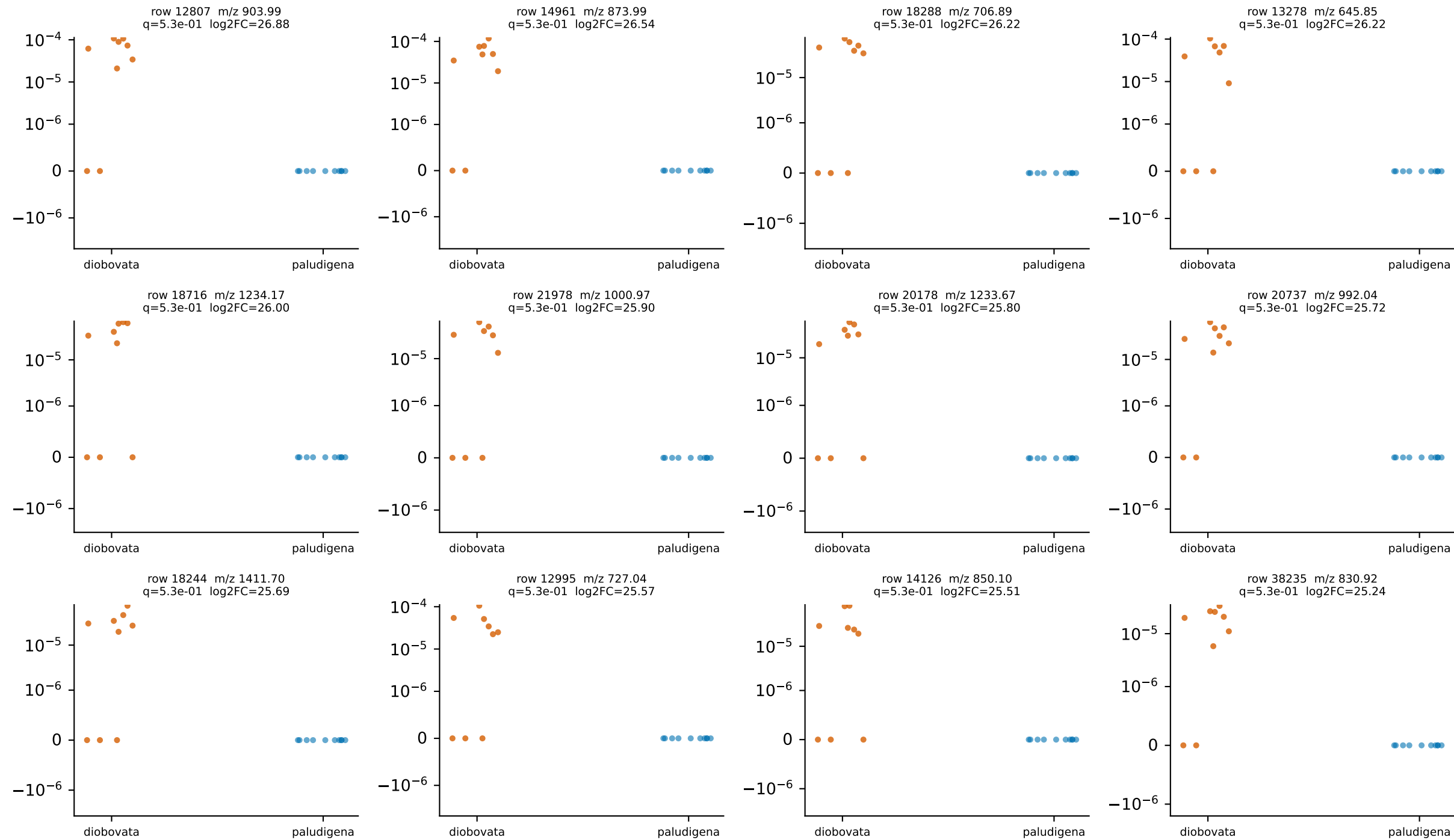
Top 12 differential features: Rhodotorula diobovata vs Rhodotorula paludigena (TSS proportion, symlog y)
