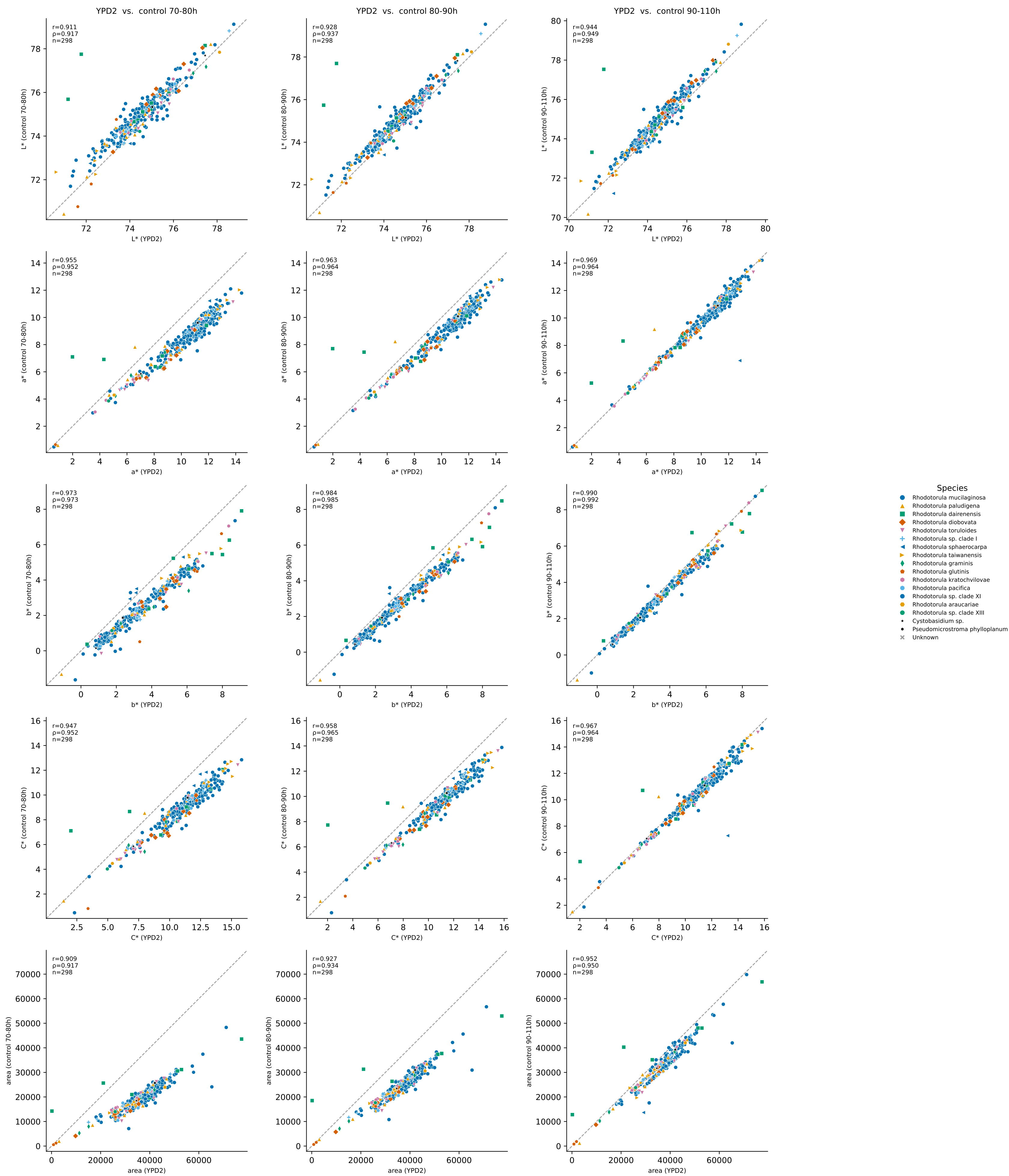
YPD2 vs. control-media timepoint windows: color & colony size (dashed = y=x)
