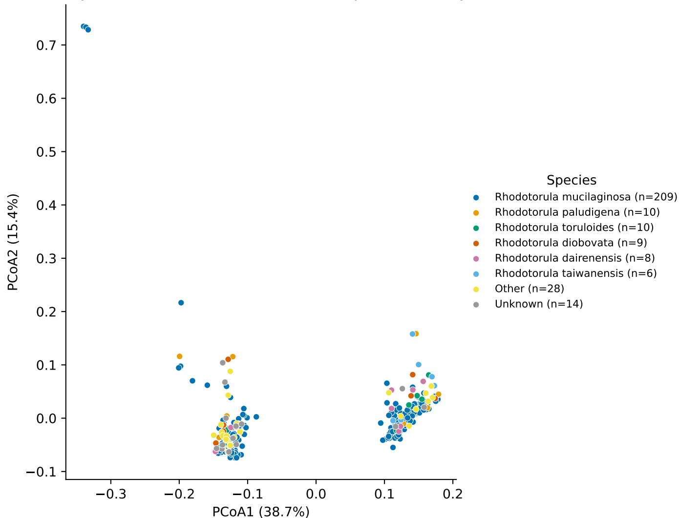
Bray-Curtis PCoA of MS2 features -- supernatant only
