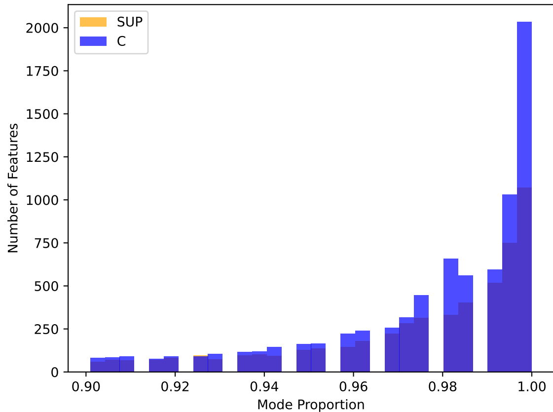
Features with mode_prop > 0.9 (Very uniform across samples)
