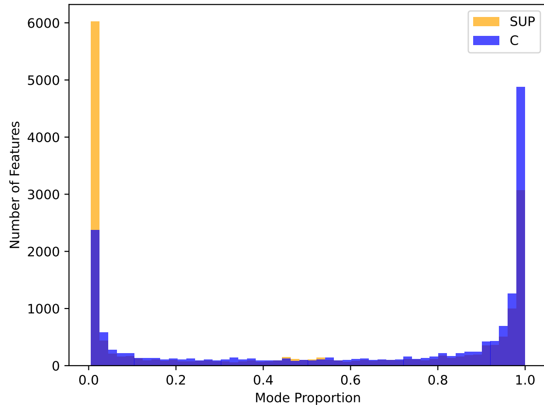
Feature Value Uniformity (Fraction of samples with mode value)
