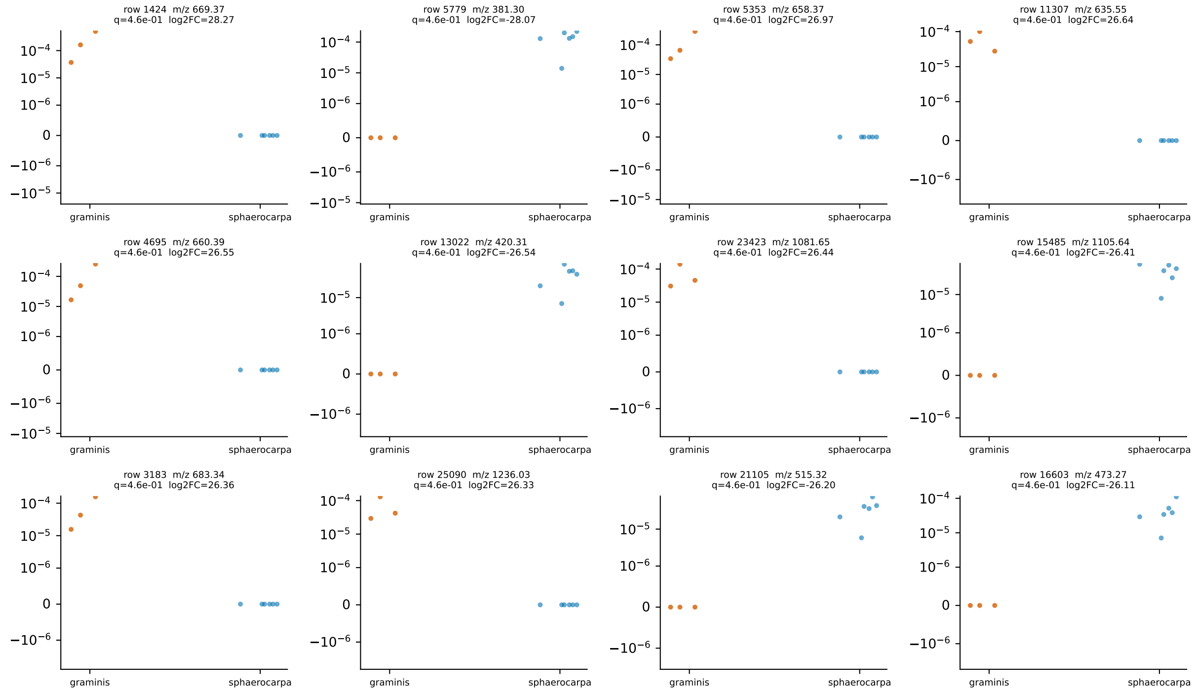
Top 12 differential features: Rhodotorula graminis vs Rhodotorula sphaerocarpa (TSS proportion, symlog y)
