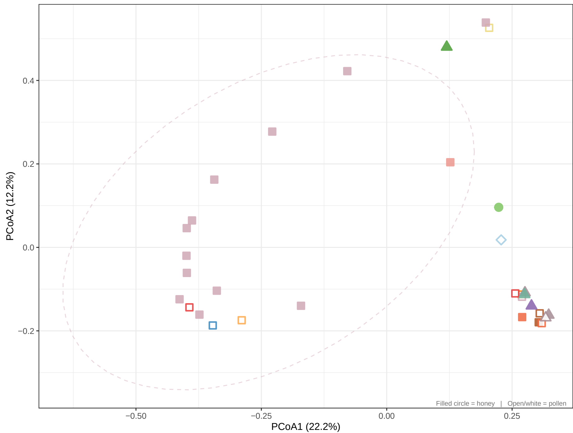
16S PCoA JACCARD
