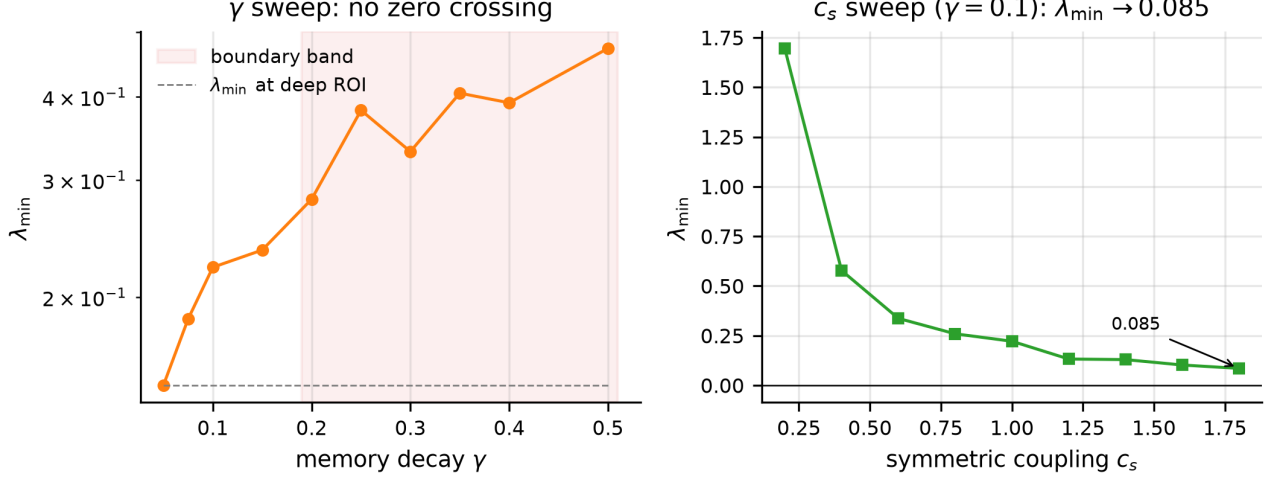
FIG. 3. Boundary sweeps along \gamma and c_s . (Left) \lambda_{\min} vs \gamma (log axis): crosses the boundary band monotonically without reaching zero. (Right) \lambda_{\min} vs c_s : monotone decrease ( 1.70 \rightarrow 0.085 ), no vanishing.
