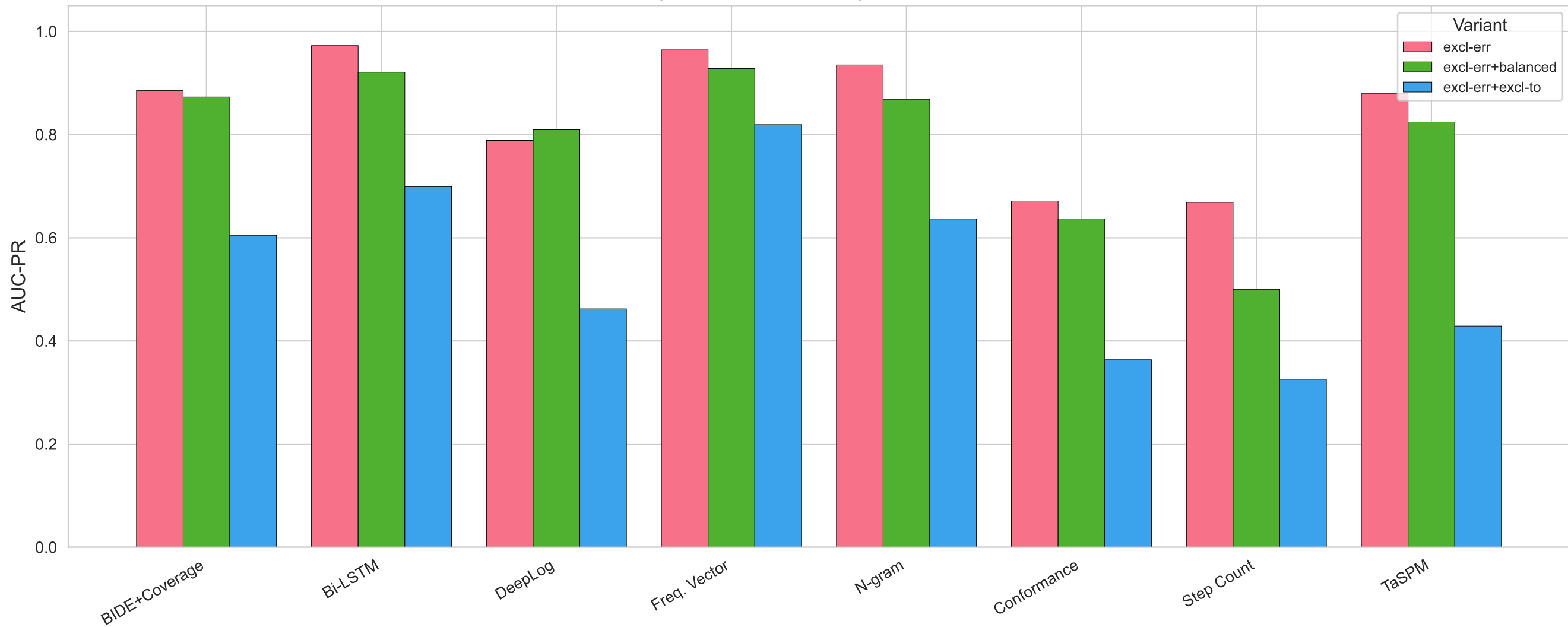
Experiment Variant Comparison at K=10
