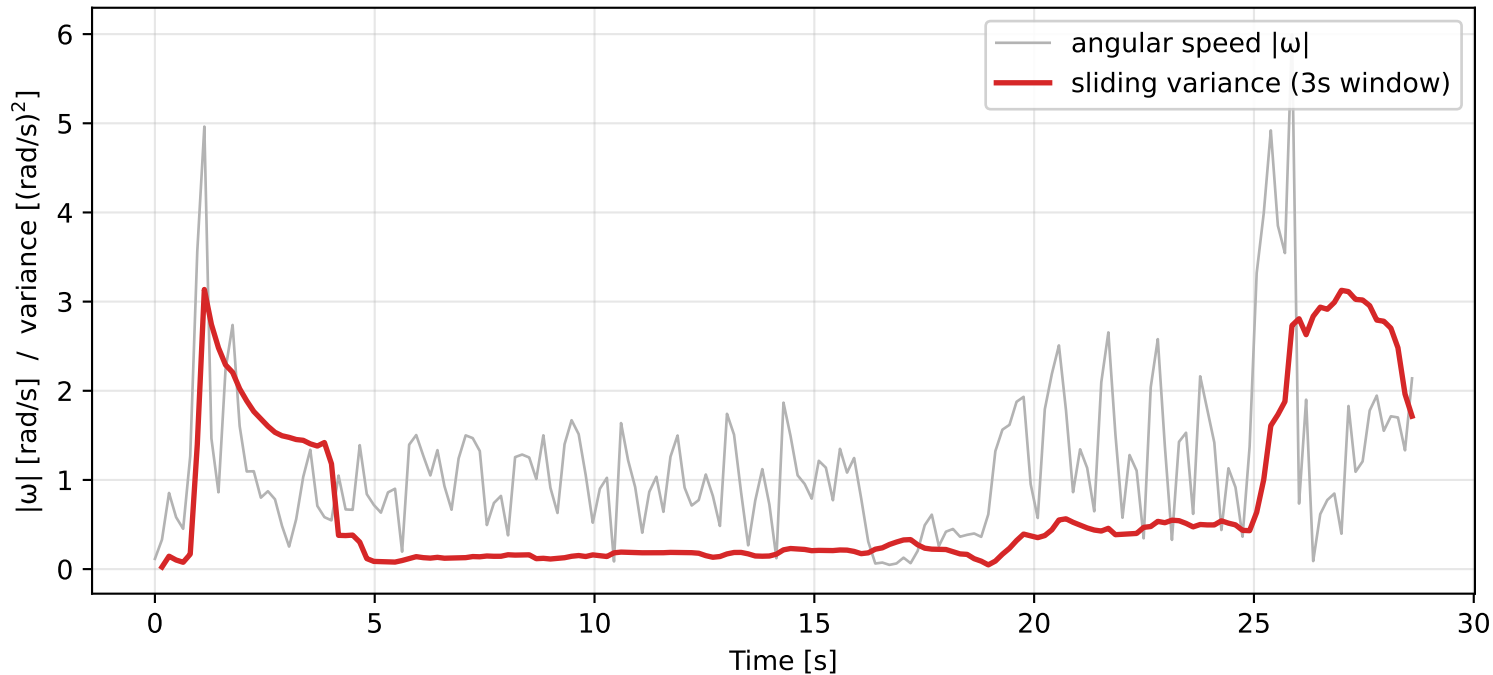
Sliding variance of gyroscope magnitude
