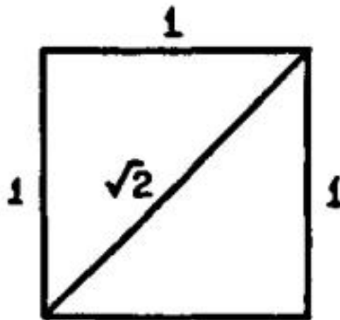
Figure 7 A square with sides of length 1
