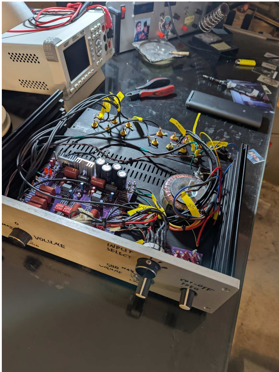
Figure 5.6: Completed preamplifier with the enclosure open during inspection.
