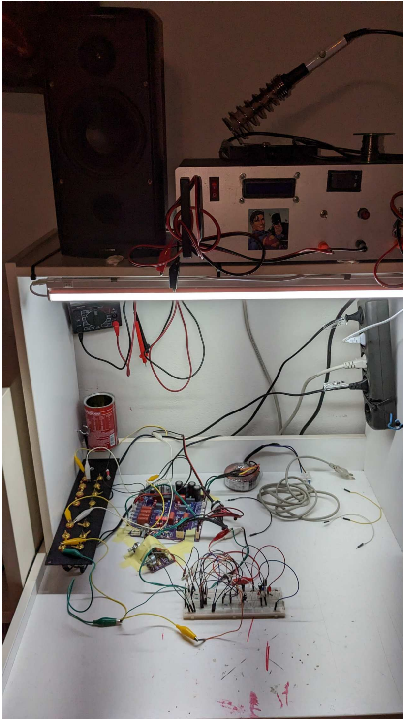
Figure 5.4: Bench wiring and integration stage during construction of the preamplifier.
