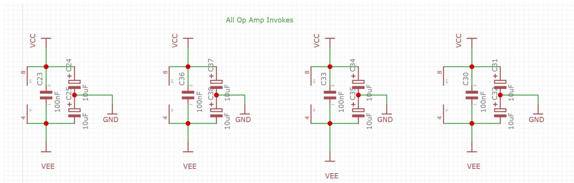
Figure 2.4: Local operational-amplifier supply decoupling and bypass arrangement.
