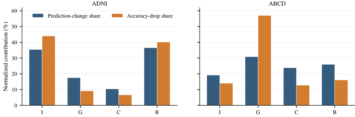
Figure 2: Normalized prediction-change and accuracy-drop shares under strict modality removal (three-seed means). I/G/C/B denote MRI/genetics/clinical/biospecimen on ADNI and imaging/genetics/cognition–health/behavior–environment on ABCD.
