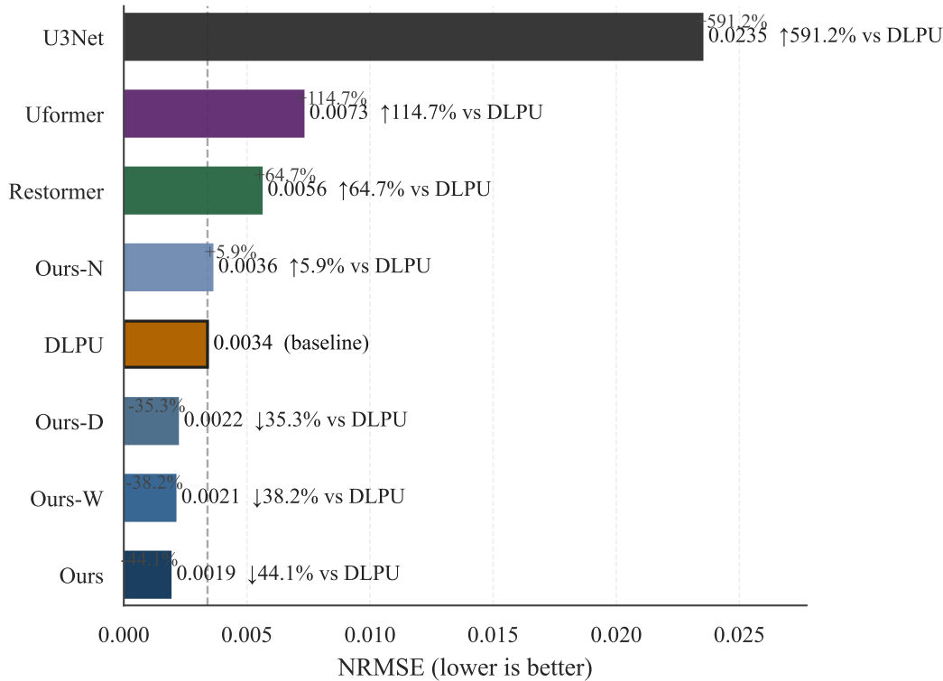
DLPU baseline NRMSE comparison against DLPU
