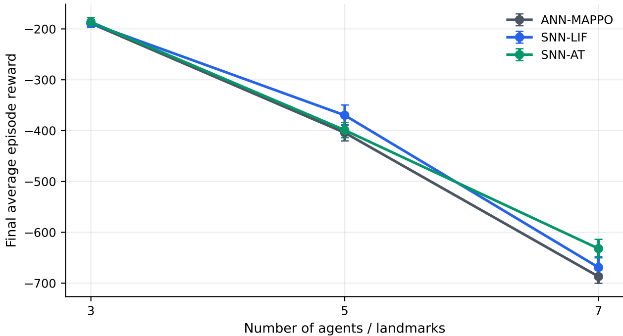
Scaling trend from 3 to 7 agents
