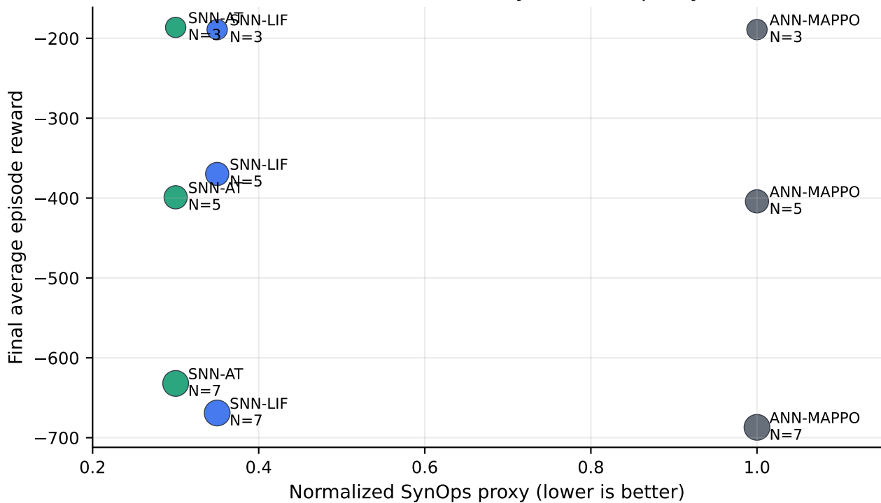
Performance-efficiency trade-off proxy
