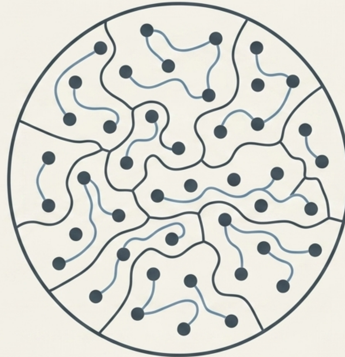
Reachability Components
