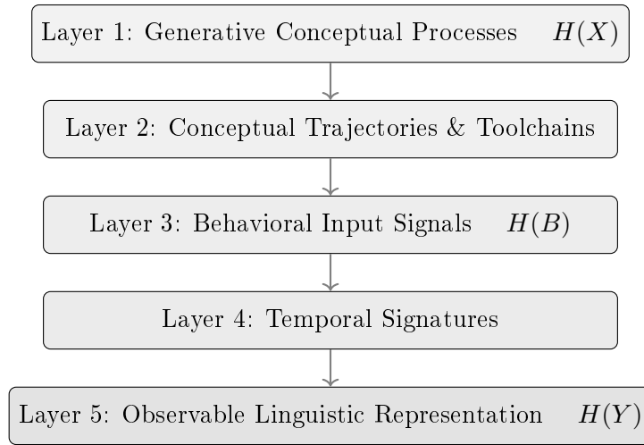
Figure 2: Five-layer model of expressive diversity in AI-mediated communication. LLMs as normalization systems act primarily at Layer 5; the deeper layers are governed by independent mechanisms and are not directly constrained by surface representation.
