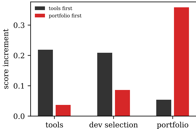
Same gap, order-dependent increments
