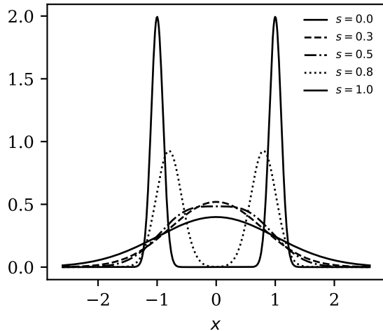
Marginals \rho_s
