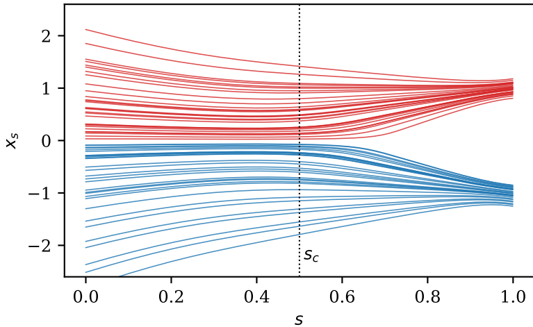
Exact-field trajectories
