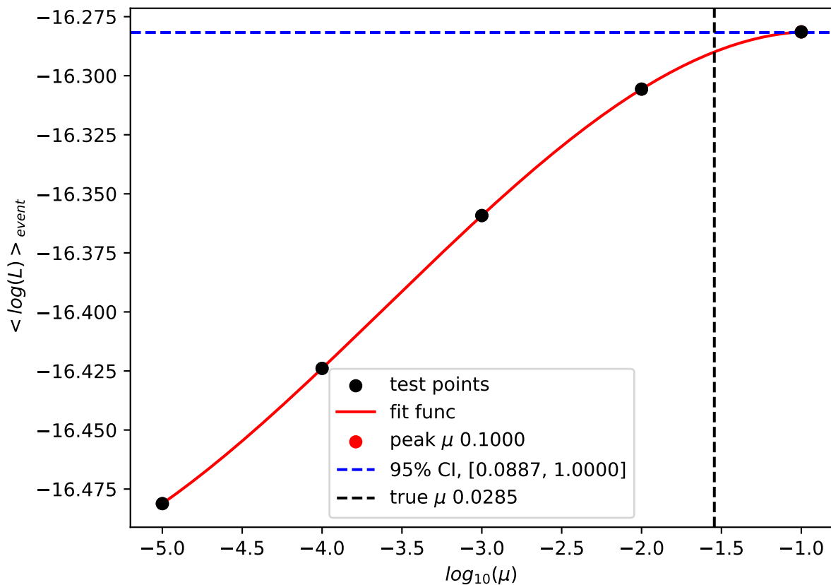
Likelihood fit at true \mu 0.0285
