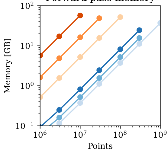
Forward pass memory
