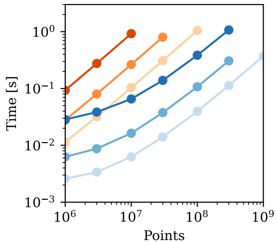
Forward pass time
