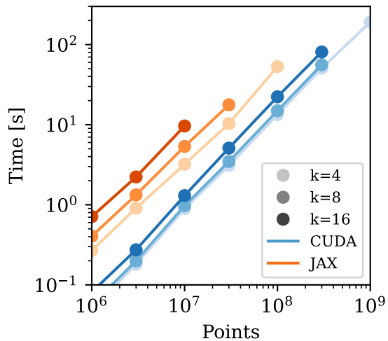
Graph build time
