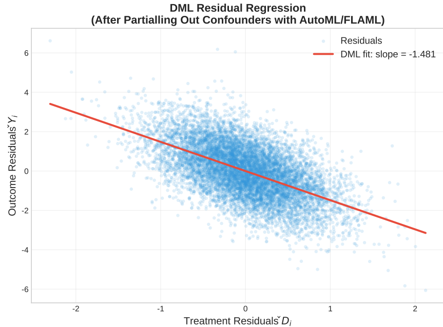
Figure 2: A scatter plot of the outcome residuals against the treatment residuals from a DML model using AutoML for the nuisance models. After partialling out the confounding effects, the simple linear relationship between the residualized variables becomes clear. The slope of this relationship is the DML estimate of the causal effect.
