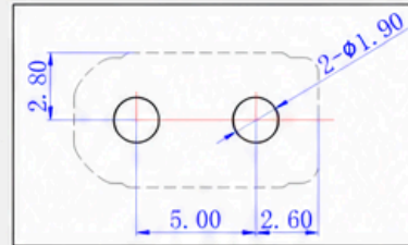
Installation Hole Diagram
