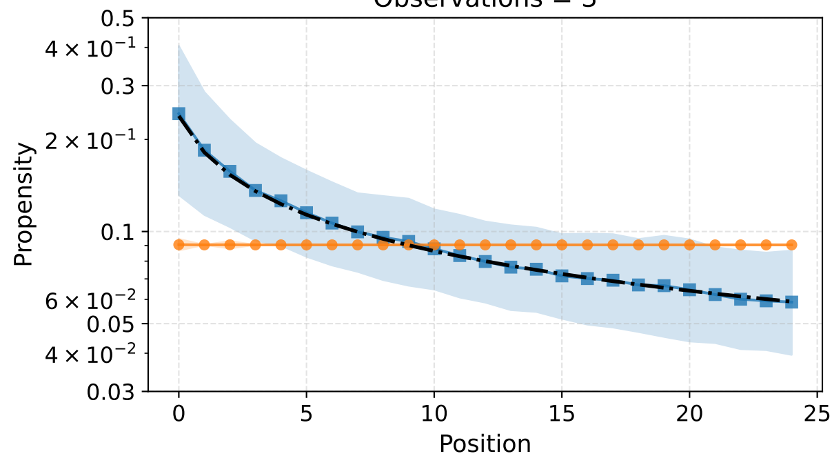
Observations = 3
