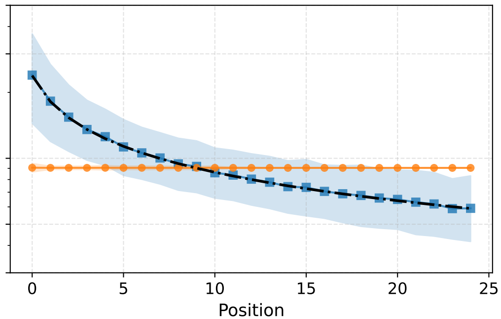
Observations = 4
