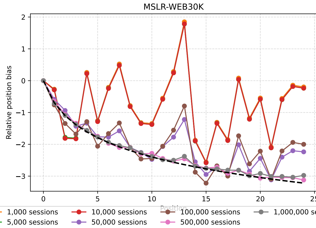
Additive Two-Tower PL Position Bias (T=1.0)
