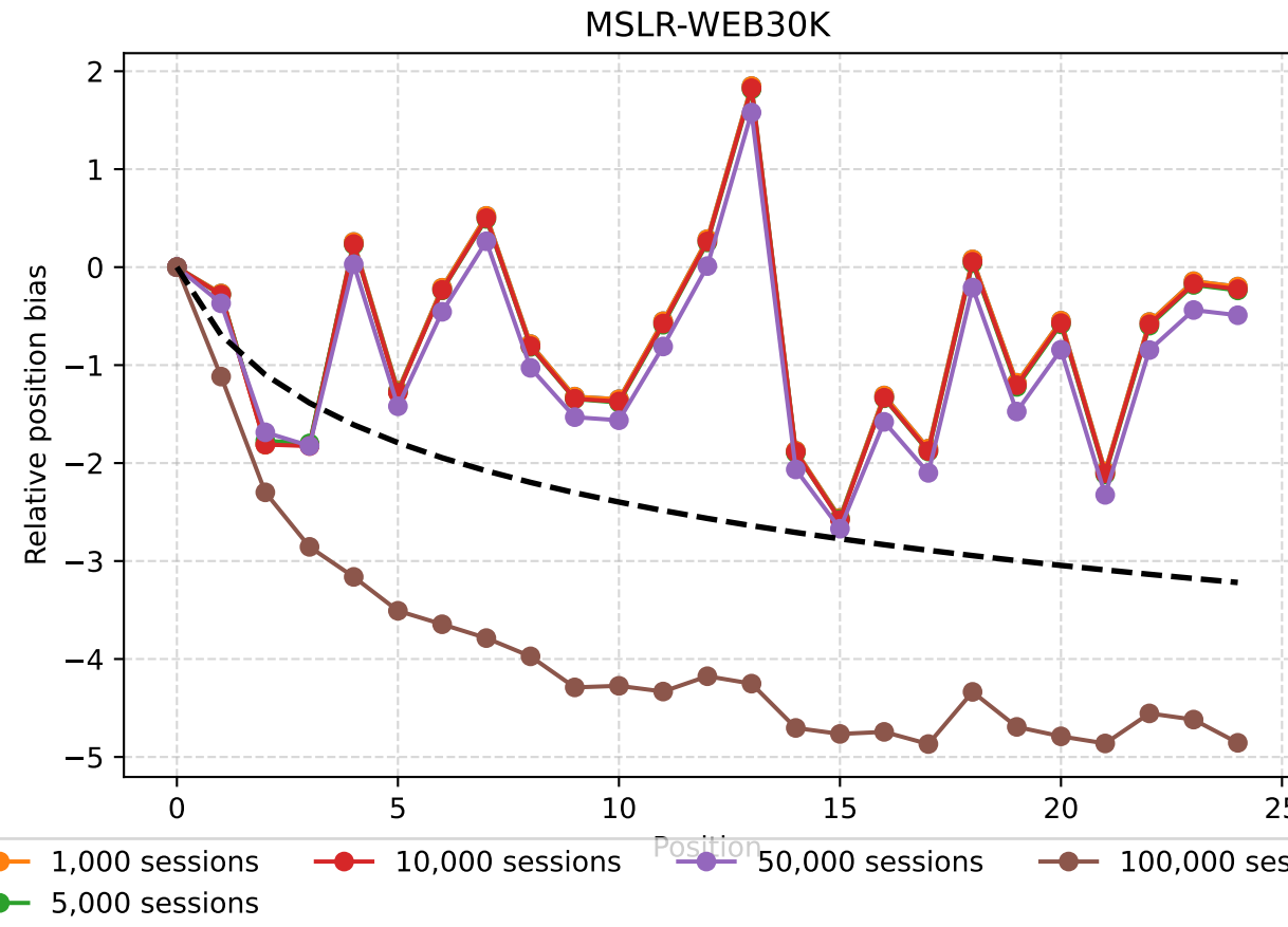
Multiplicative Two-Tower PL Position Bias ( T=0.5 )
