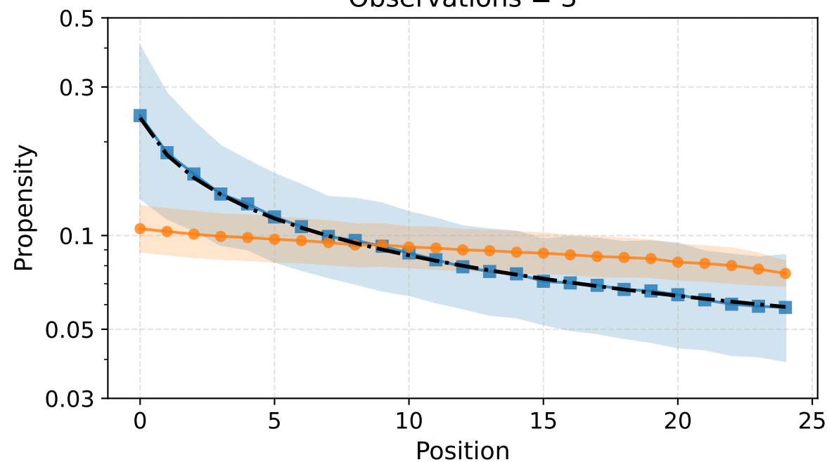
Observations = 3
