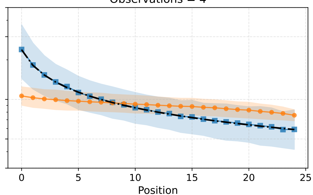
Observations = 4
