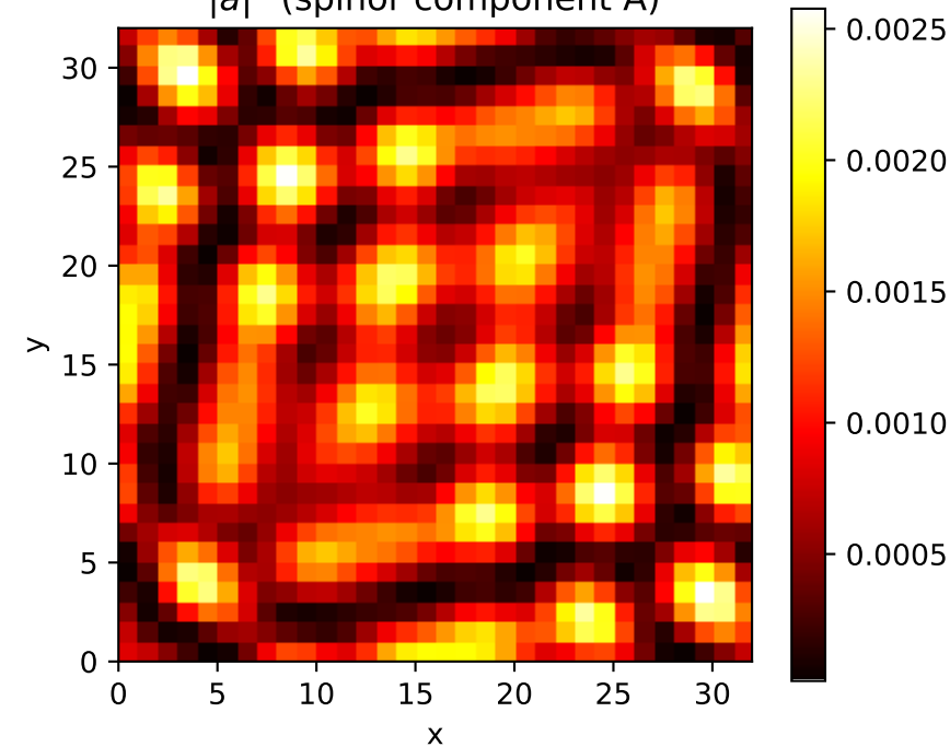
|a|^2 (spinor component A)
