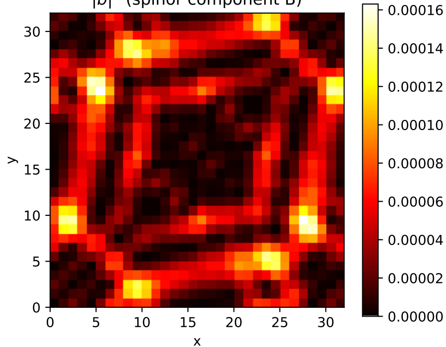
|b|^2 (spinor component B)
