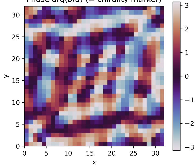
Phase \arg(b/a) (= chirality marker)
