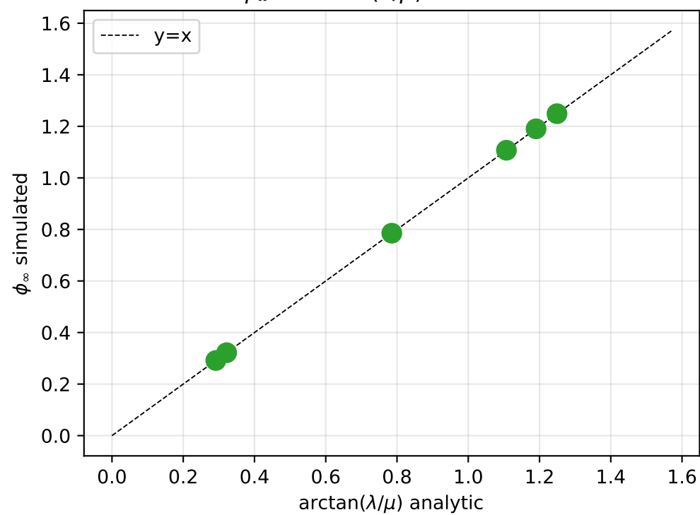
Test 4: Inertial relaxation \phi_\infty = \arctan(\lambda/\mu) to \sim 10^{-6}
