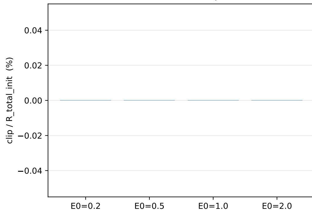
Test 1: Conservation flux zero-sum: \leq 1e-17 , clip \sim structural
