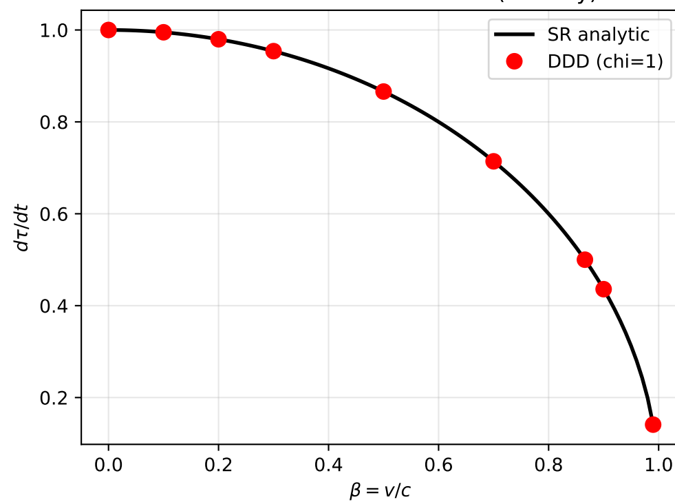
Test 5: SR recovered at chi=1 (identity)
