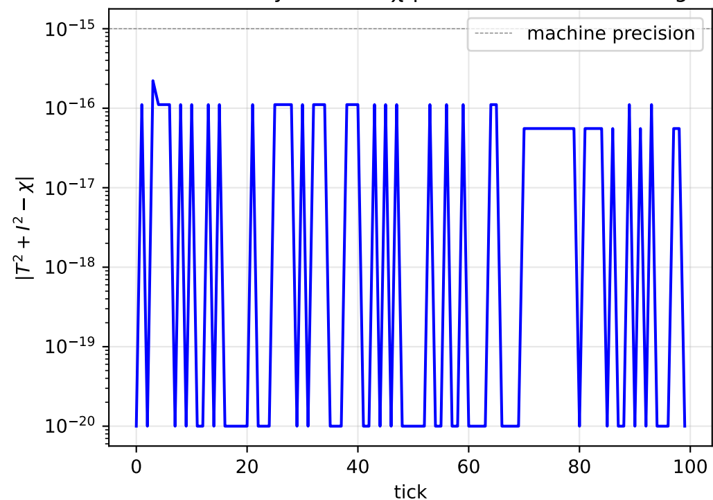
Test 2: Identity T^2 + I^2 = \chi preserved under drainage
