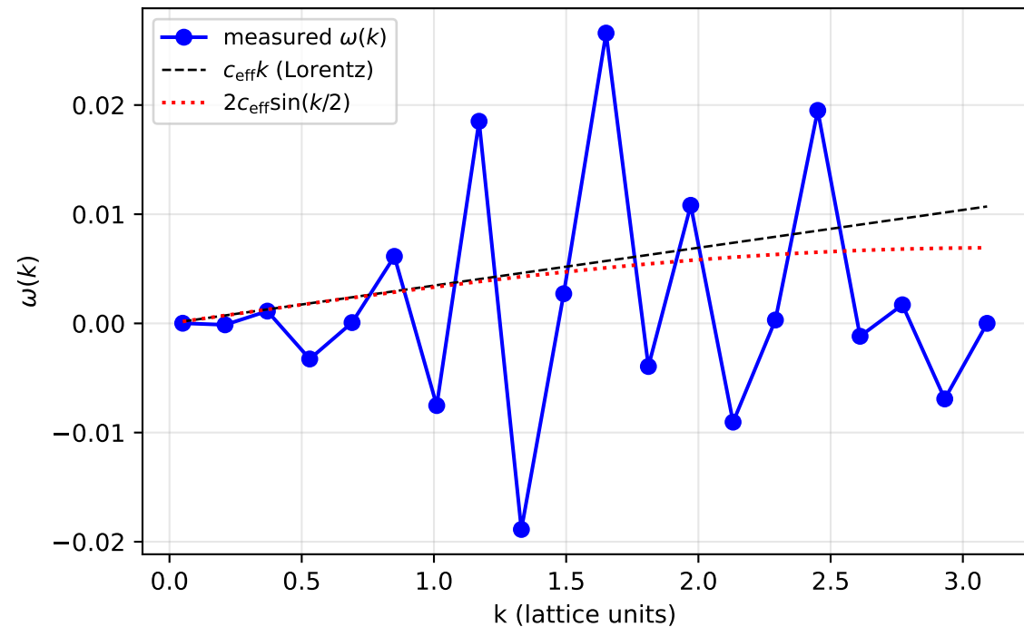
Dispersion relation, c_{\text{eff}} = 0.003
