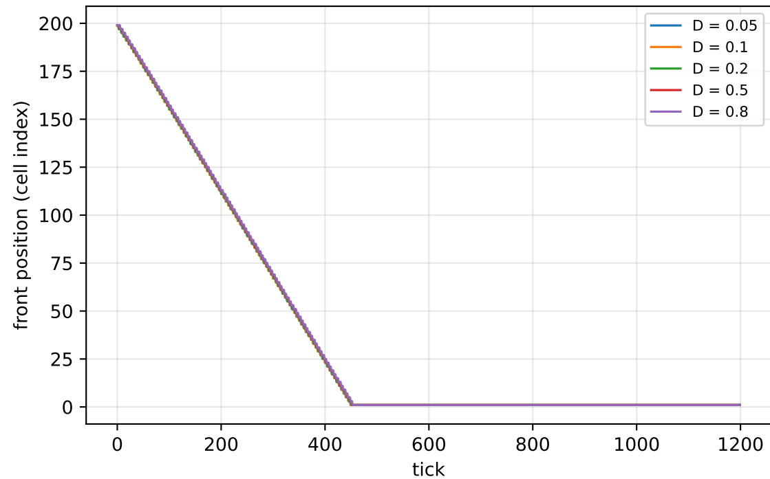
Front trajectory vs initial deficit amplitude
