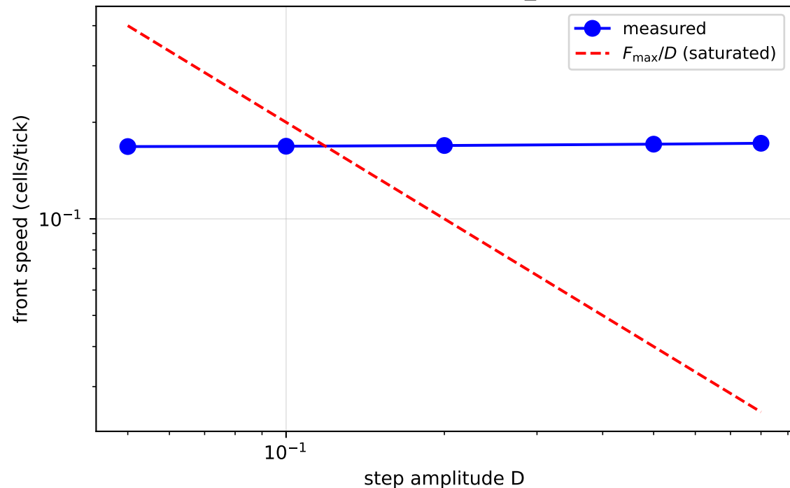
Front speed vs amplitude ( F_{\max} = 0.02 )
