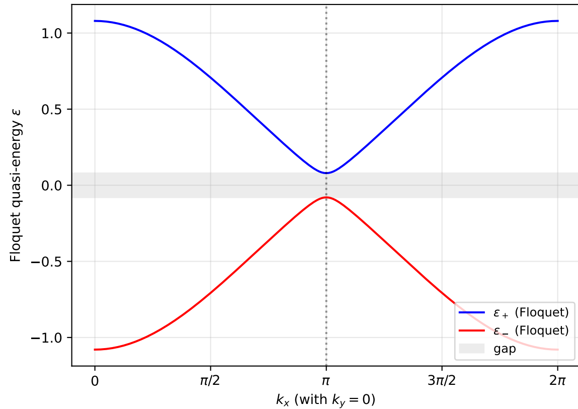
Full quasi-energy band structure
