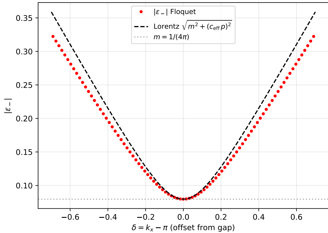
Zoom on the gap at (\pi, 0) with Lorentz fit
