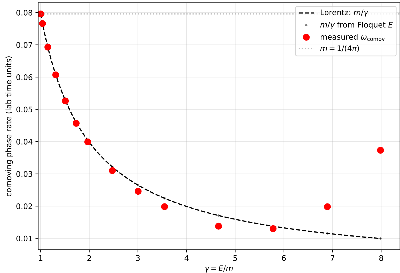
Operational kinematic clock rate vs Lorentz prediction
