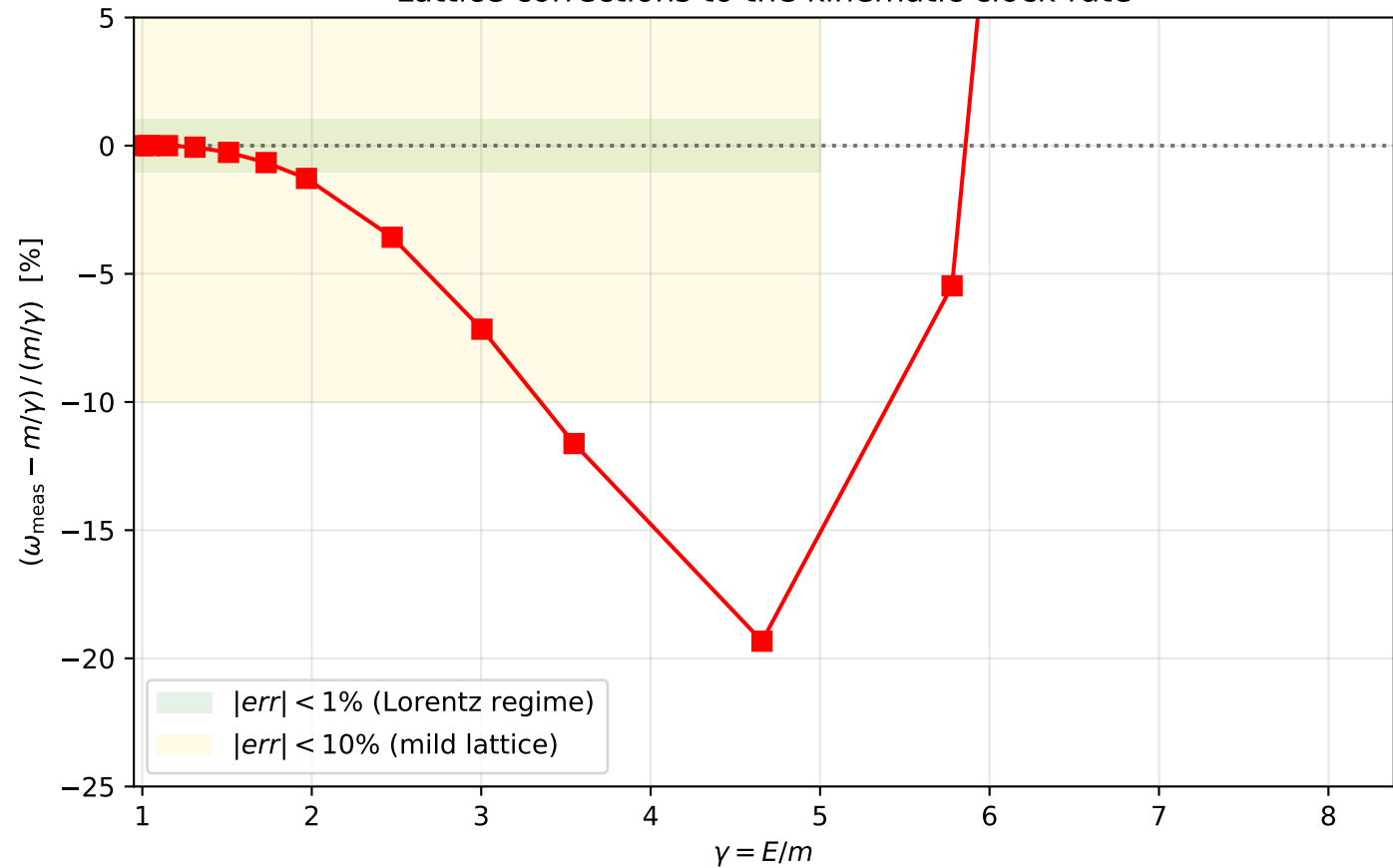
Lattice corrections to the kinematic clock-rate
