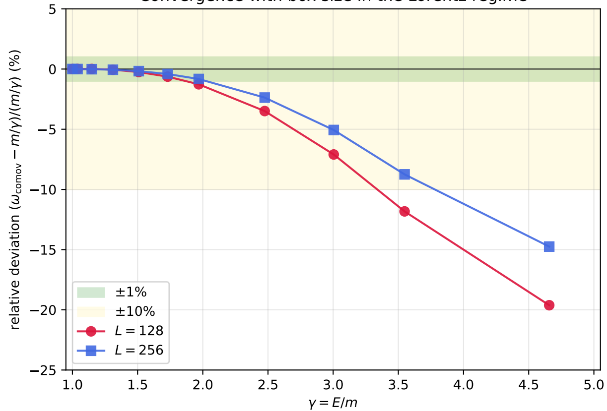
Convergence with box size in the Lorentz regime
