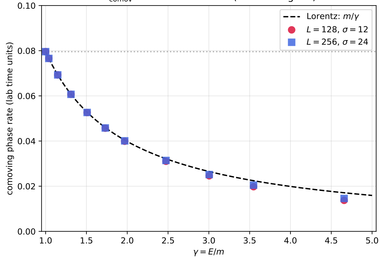
\omega_{\text{comov}}: L = 128 \text{ vs } L = 256 \text{ (Lorentz regime)}
