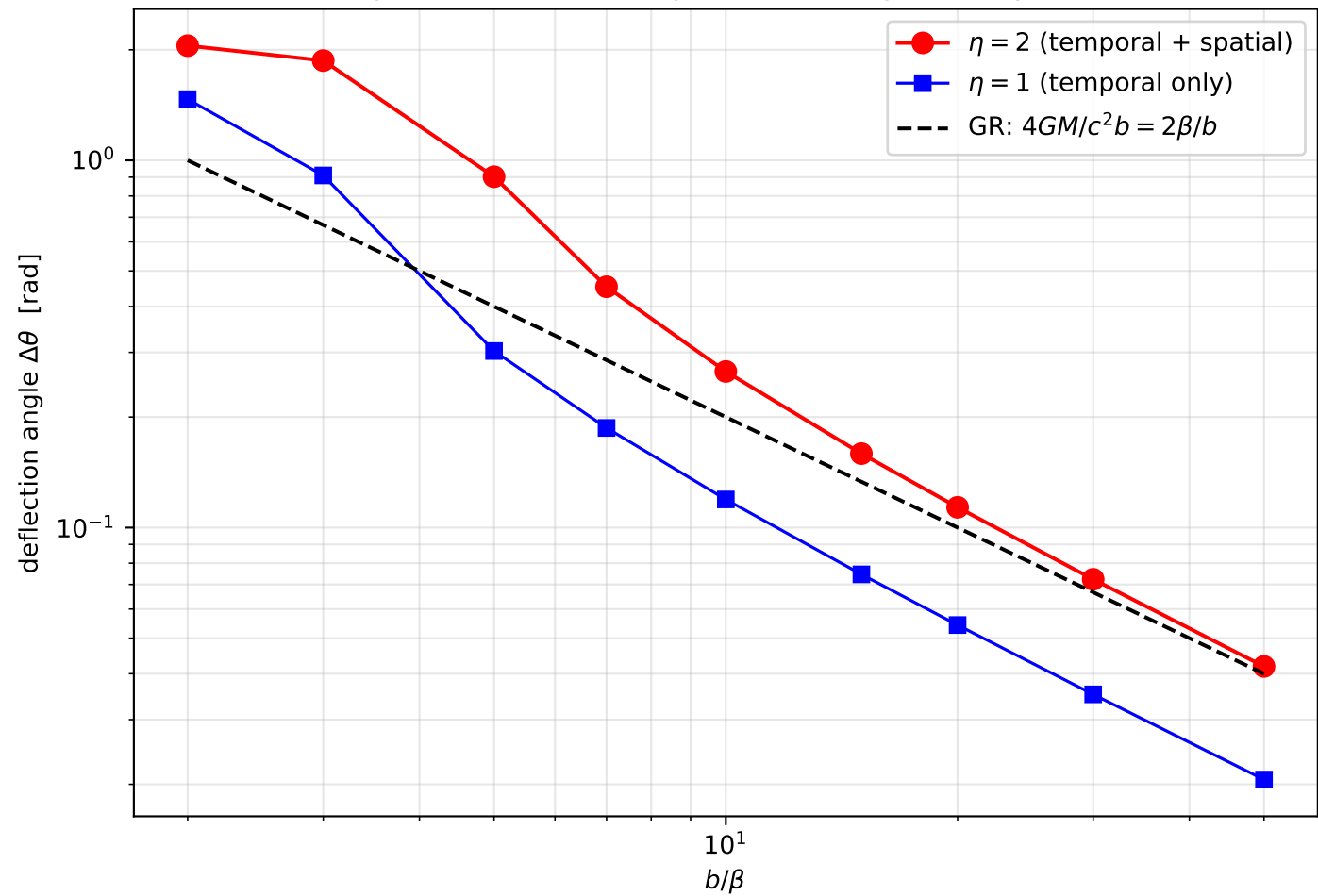
Light deflection through the static spherical profile
