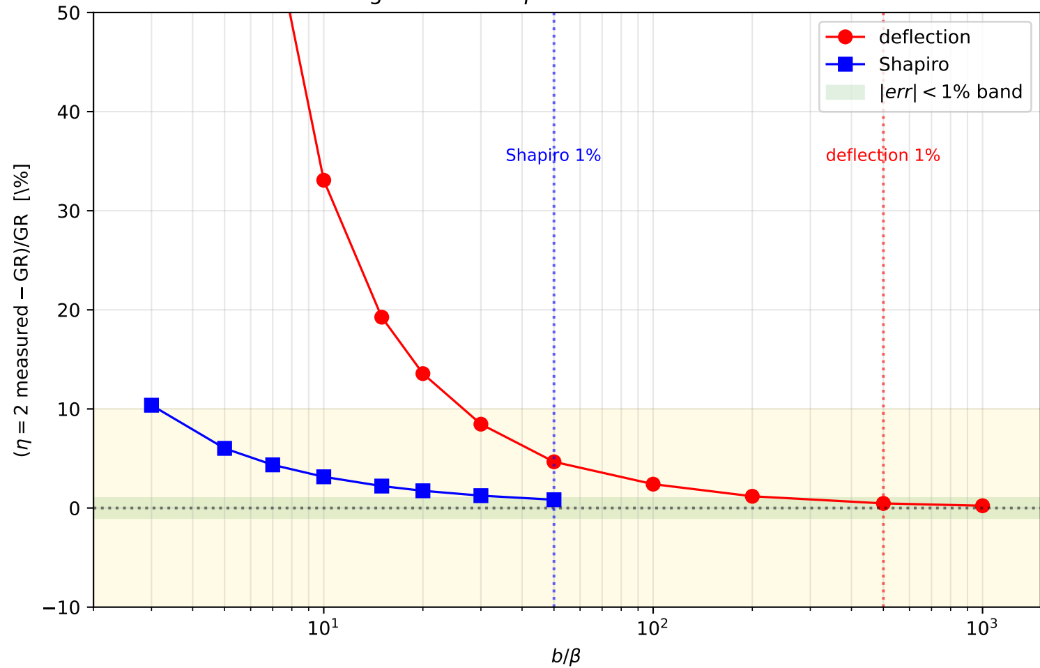
Convergence of the \eta = 2 ansatz to weak-field GR
