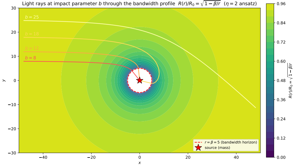
Figure 1: Schematic of light rays at impact parameters b traversing the static spherical bandwidth profile R(r)/R_0 = \sqrt{1 - \beta/r} of Paper II. The dashed circle marks the bandwidth horizon r = \beta where R \rightarrow 0 and the eikonal approximation fails. Rays are bent by the gradient of \ln n(r) , with n = (R_0/R)^\eta .
