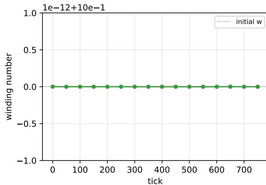
Test 2: vortex stability residual = 0.0000
