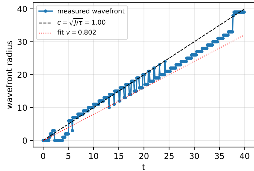
Test 1: wave propagation
