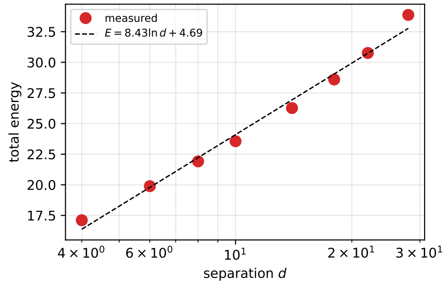
Test 3: vortex-antivortex (Coulomb-like)
