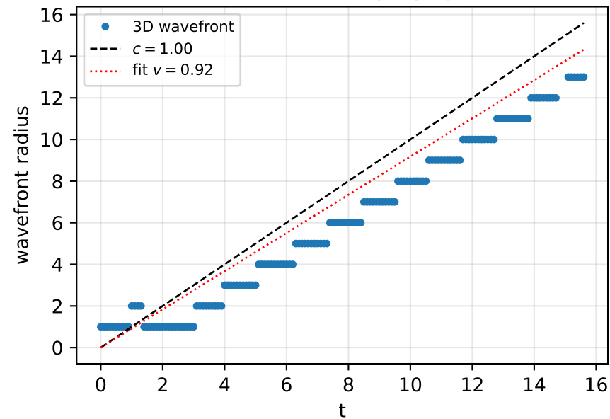
Test 1 (3D): wave propagation
