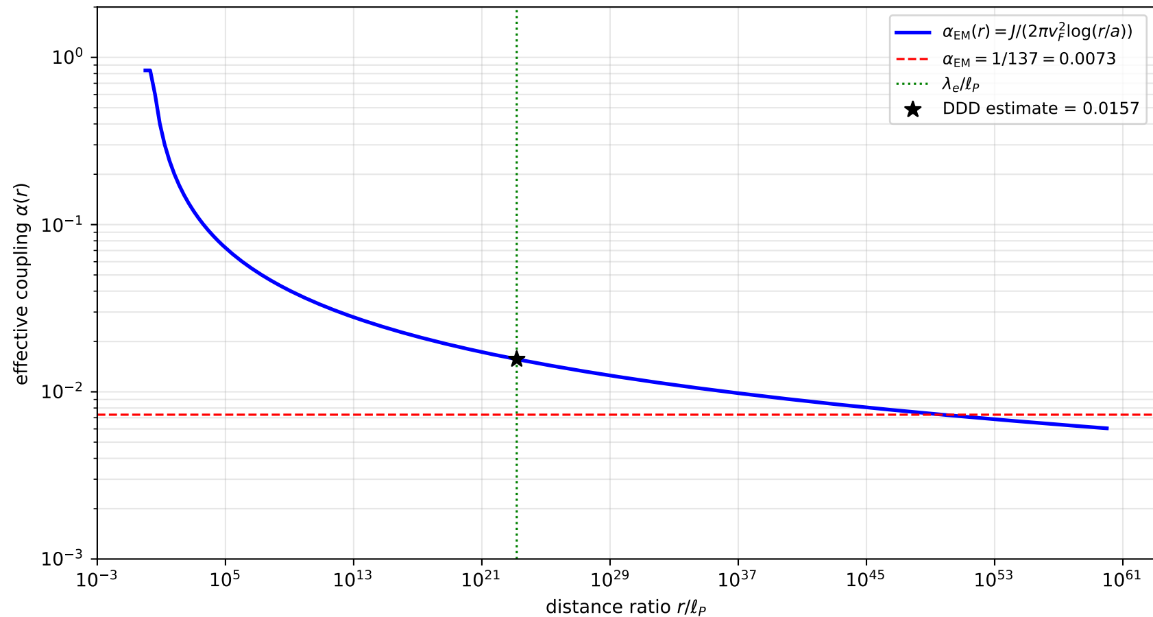
DDD running coupling vs CODATA \alpha_{\text{EM}} Estimate: \alpha_{\text{DDD}} = 0.0157 , factor 2.15 of truth
