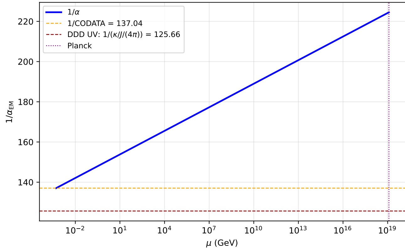
(b) 1/\alpha shows linear running in \log(\mu)
