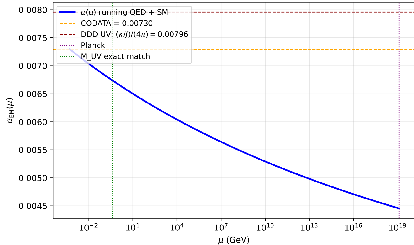
(a) RG running of \alpha_{\text{EM}}
