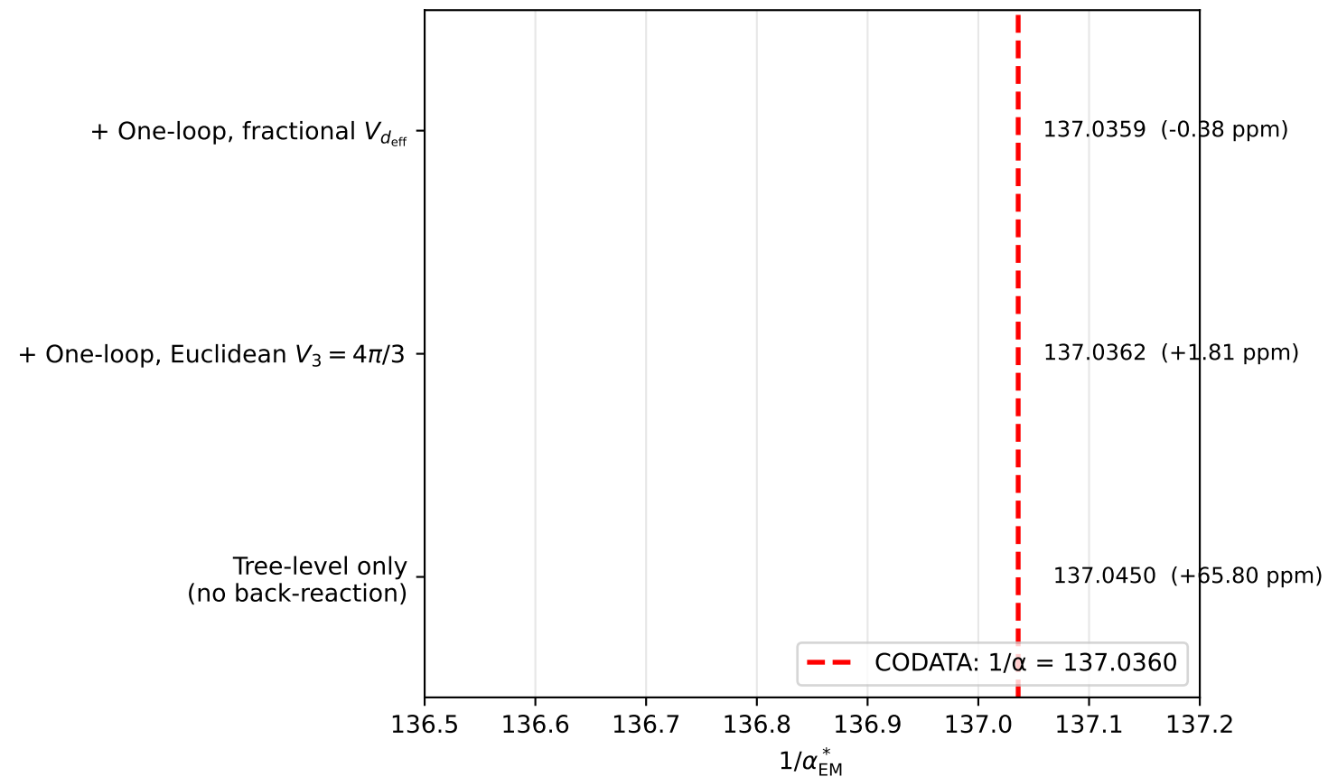
Self-consistent fixed point of \alpha_{\text{EM}}
