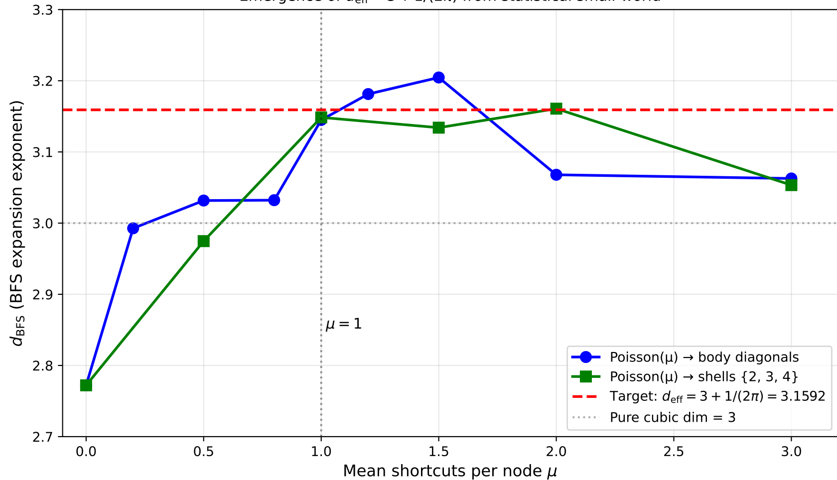
Emergence of d_{\text{eff}} = 3 + 1/(2\pi) from statistical small-world
