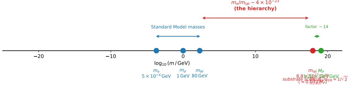
Figure 1: Scale hierarchy interpretation. Standard Model masses sit at \sim 10^{-3} to 10^2 GeV, \sim 23 orders of magnitude below the substrate mass scale m_{\text{lat}} \approx 0.072 M_P \approx 8.8 \times 10^{17} GeV. The substrate is itself a factor \sim 14 below the Planck mass. At the substrate scale, gravity and electromagnetism are comparable ( \alpha_G/\alpha_{\text{EM}} = 1/\sqrt{2} ); the observed weakness of gravity for ordinary particles is a consequence of the ratio m_e/m_{\text{lat}} \sim 4 \times 10^{-23} , not of any fundamental weakness of the gravitational coupling.
