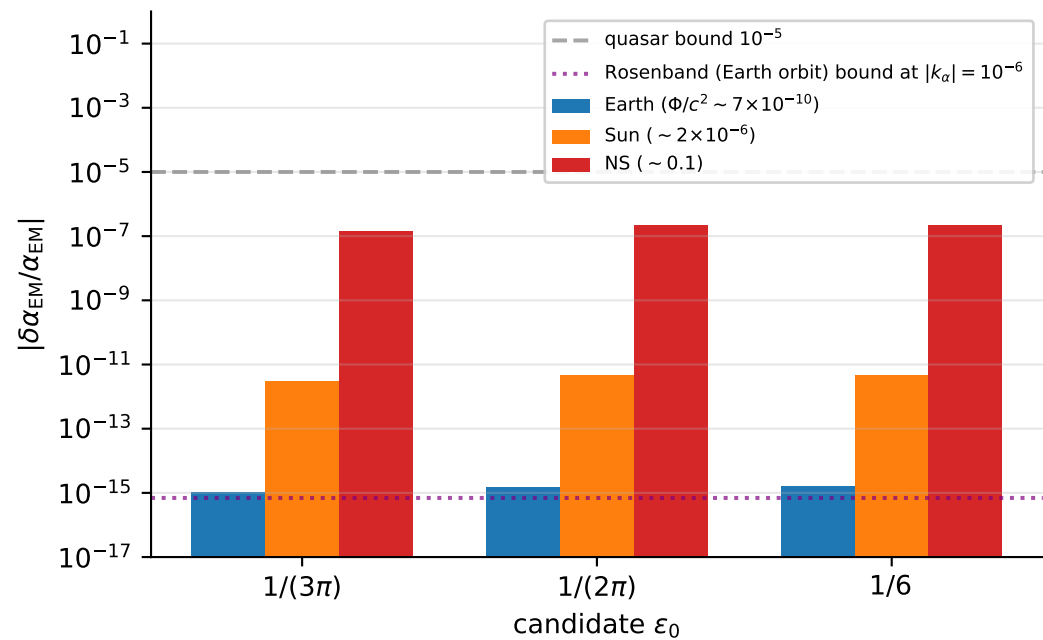
(b) Predicted spatial shift in \alpha_{\text{EM}}
