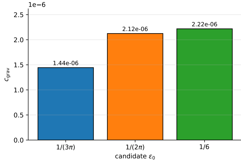
(a) Cross-coupling prefactor c_{\text{grav}} for the three candidates
