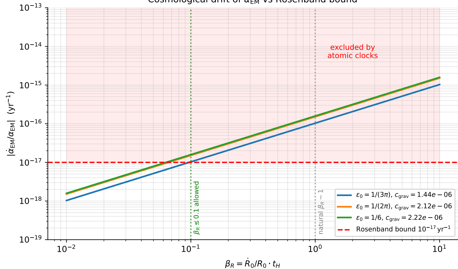
Cosmological drift of \alpha_{\text{EM}} vs Rosenband bound
